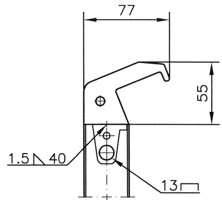
Detail Z
