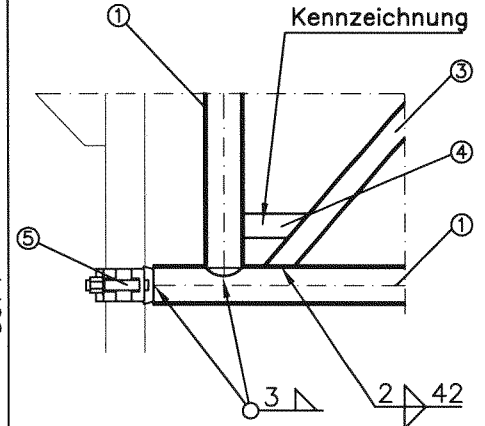
Detail Y \curvearrowright 90^\circ
