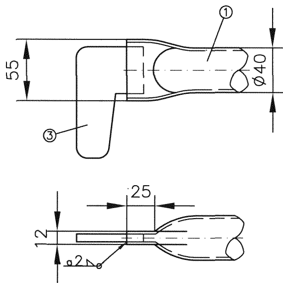
Detail X
