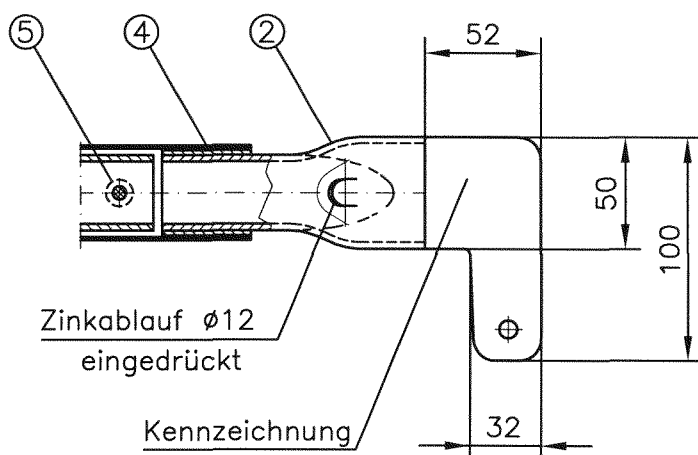
Detail X
