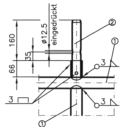
Detail Z \curvearrowright 90^\circ
