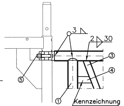
Detail X \curvearrowright 90^\circ
