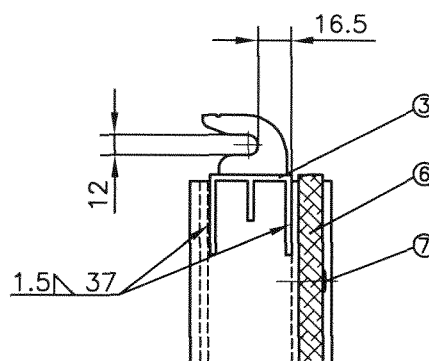
Detail Z
