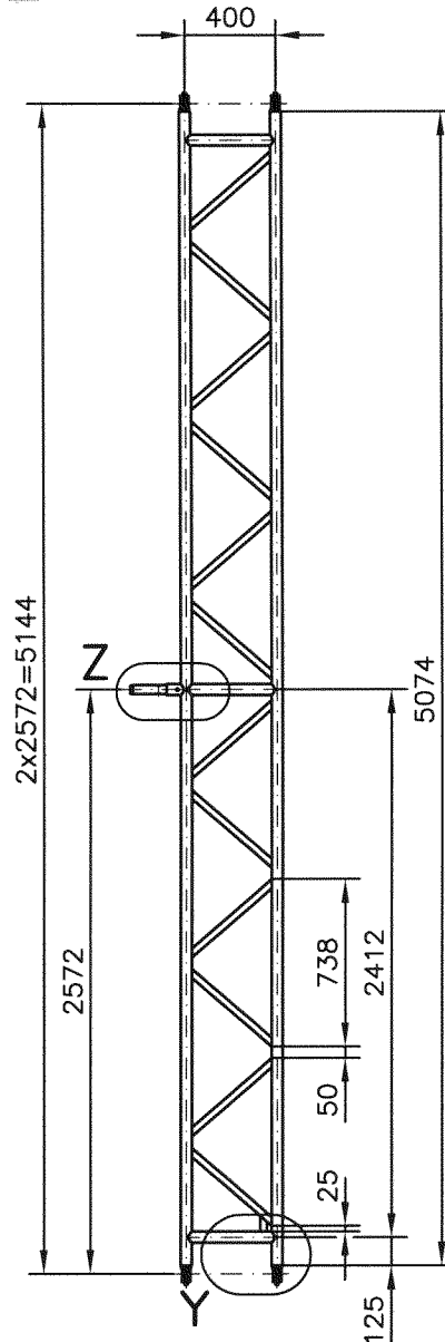
Detail Y \curvearrowright 90^\circ
