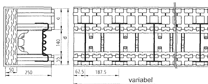
Sturzstein "S"
