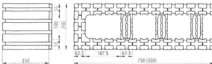
25er-Innenwand-Endelement
