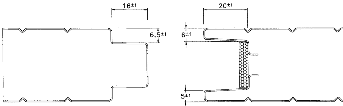
Detail B
