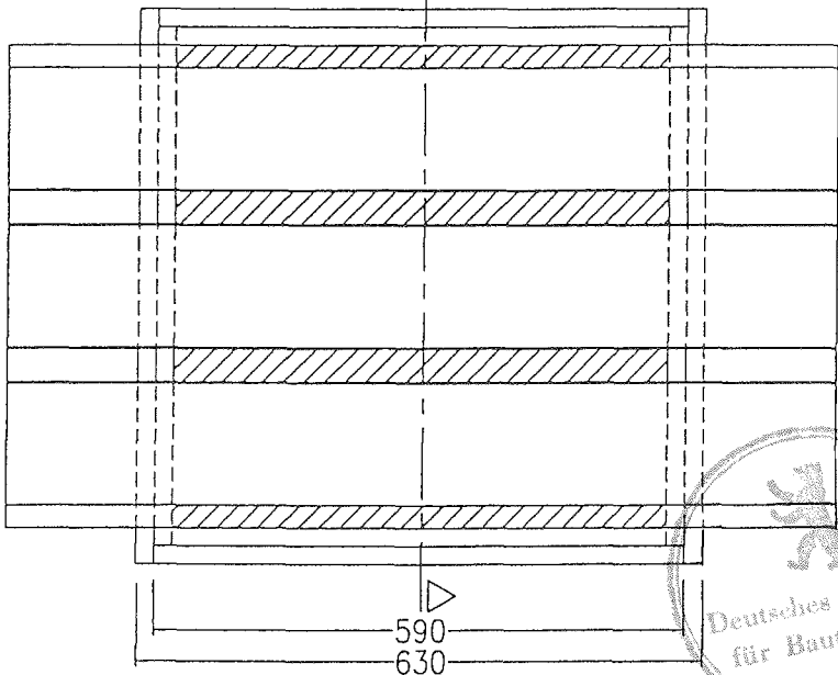
System KBA-30/40 KBC-40
