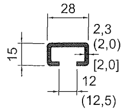
HTA 28/15 S235JR A4, DX**, FA, HCR*
