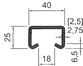
HTA 40/25 S235JR A4, DX**, FA, HCR
