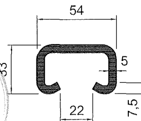
HTA 54/33 S355MC A4, DX, FA, HCR
