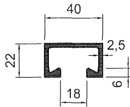
HTA 40/22 S235JR A4, FA, HCR
