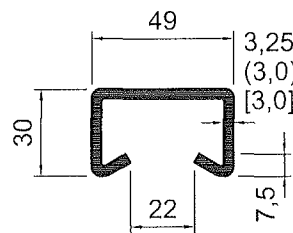
HTA 49/30 S235JR A4, DX**, FA, HCR*
