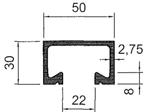
HTA 50/30 S235JR A4, FA, HCR
