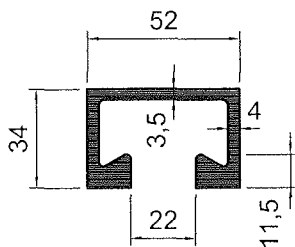
HTA 52/34 S235JR A4, FA, HCR
