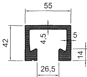
HTA 55/42 S275JR
