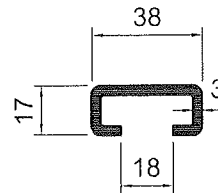
HTA 38/17 S235JR A4, DX, FA, HCR
