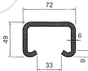
HTA 72/48 S235JR A4, FA, HCR
