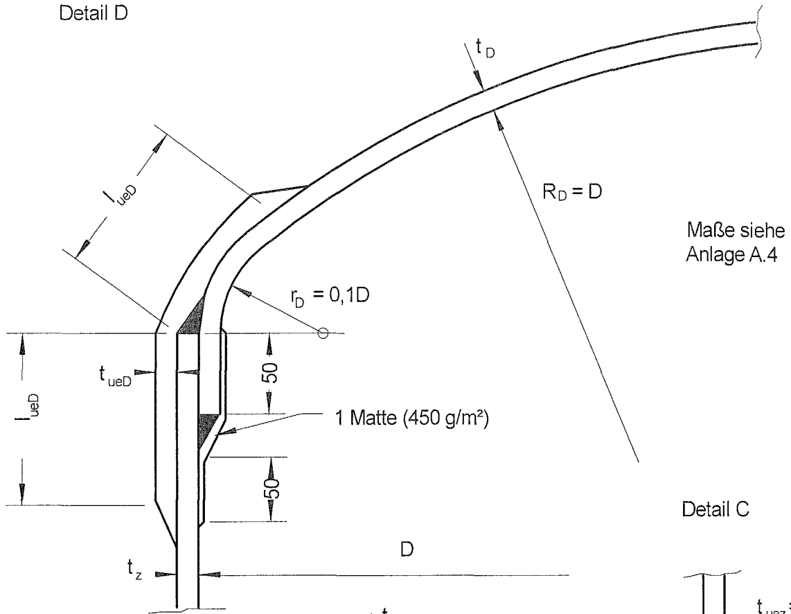
Detail D (Alternative)
