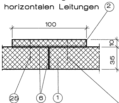
Detail C
