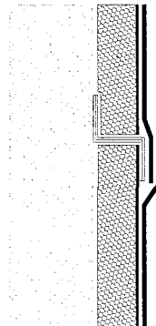
Fig. 9: Intermediate fixing (vertikal) for insulated components with metal profile (Z-Profile)
