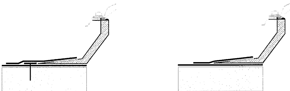
Fig. 17: Connection to the dome light with PVC-frame
