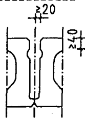
Fugendetail
