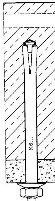
Through-set installation external thread
