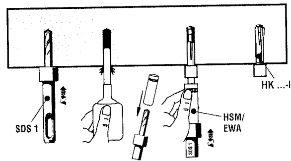
Setting of HK...-I with machine setting tool
