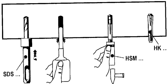
Setting of HK with hand setting tool
