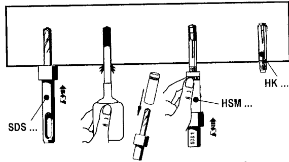
Setting of HK with machine setting tool
