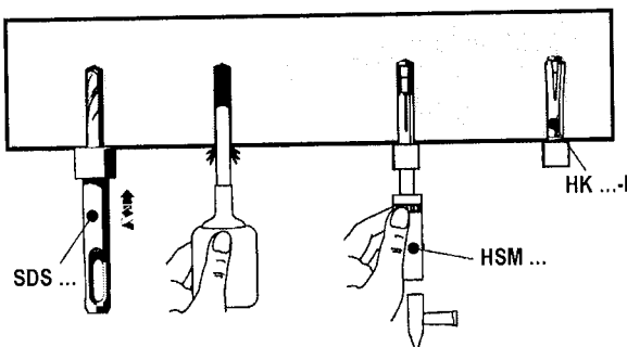
Setting of HK...-I with hand setting tool
