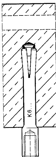
Pre-set installation internal thread
