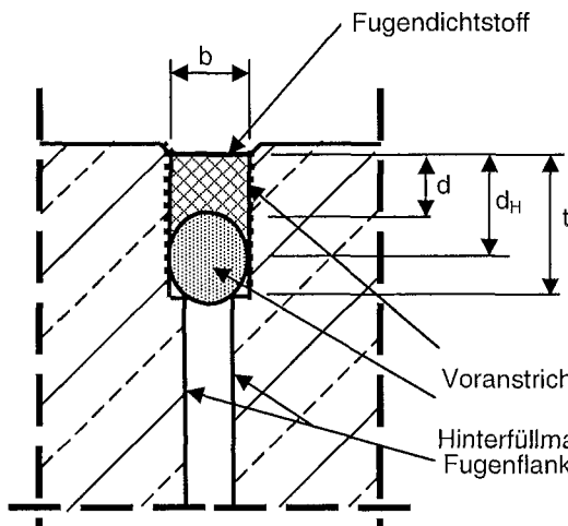
Beton/Polymerbeton – Beton
