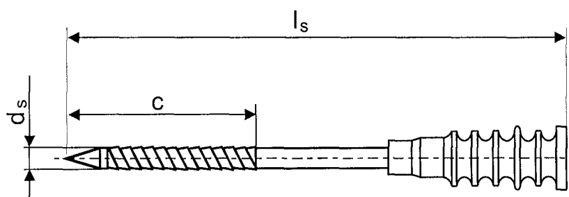
Nail with an integrally moulded plastic head
