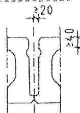
Fugendetail
