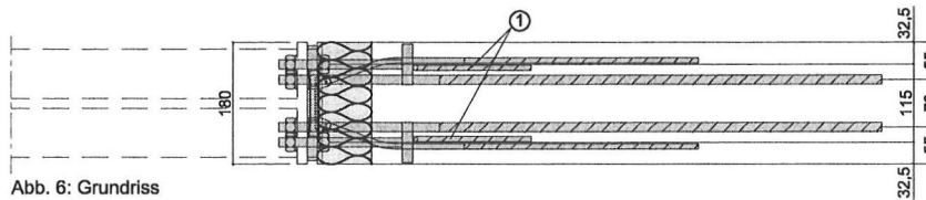
Abb. 6: Grundriss
