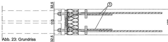
Abb. 23: Grundriss
