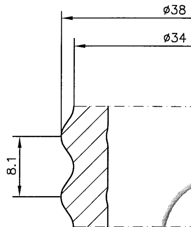
Detail X
