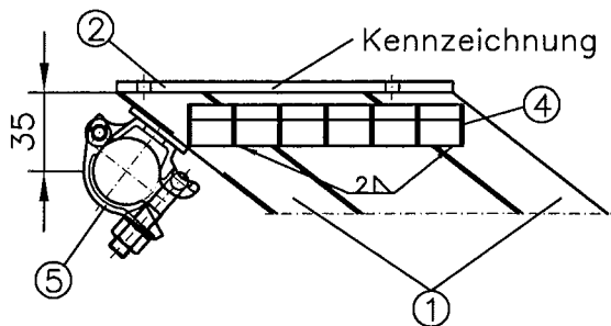
Detail X
