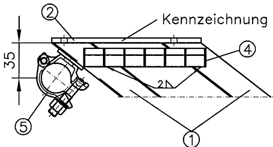
Detail X
