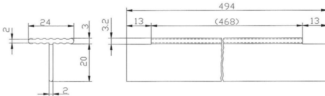
Vertical connection profil "PVC Verbindungsleiste" (dimensions in millimetres)
