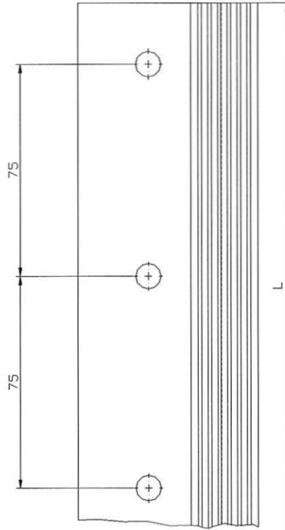
Vertical connection profil "PVC Verbindungsleiste" (dimensions in millimetres)
