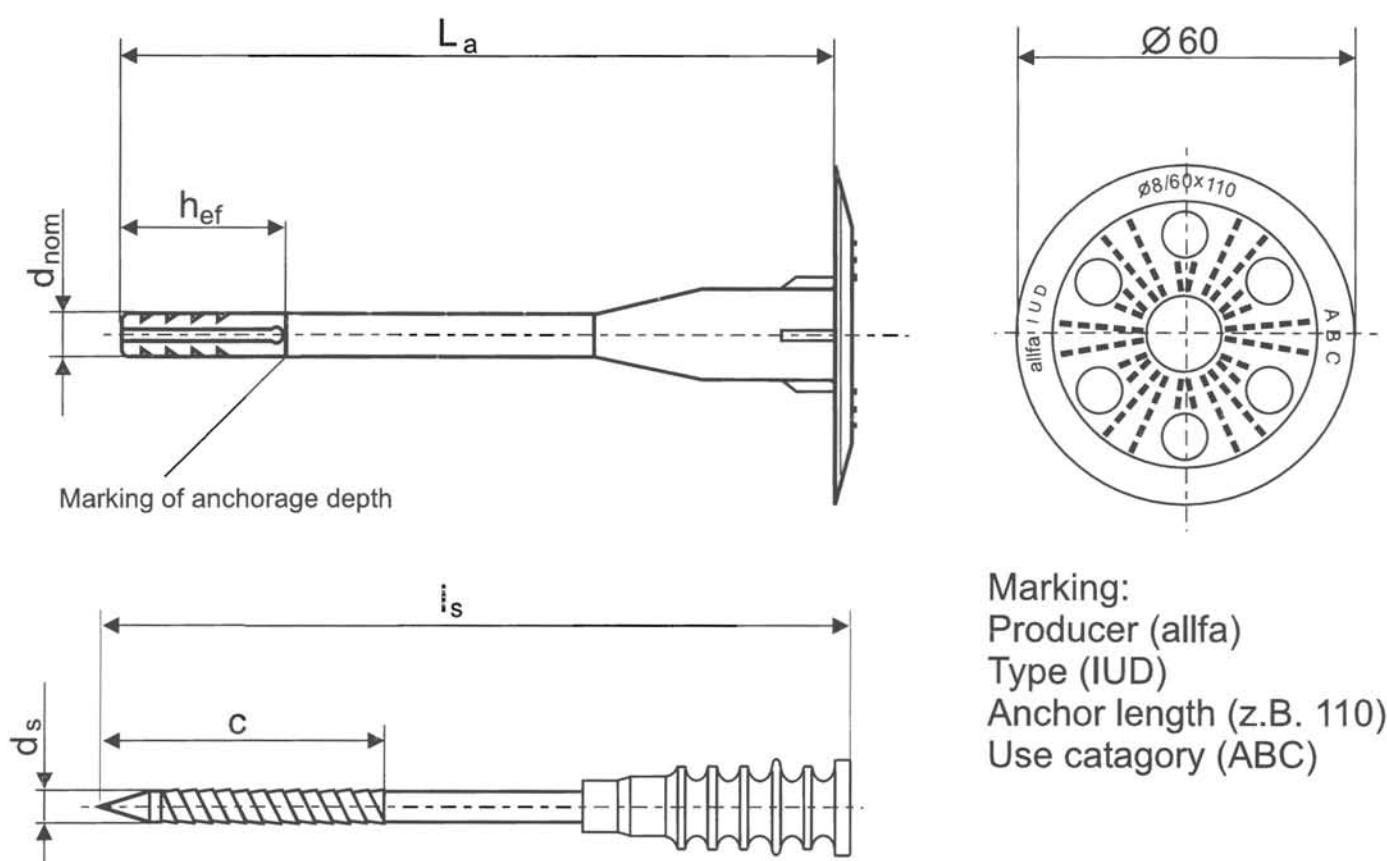
Nail with an integrally moulded plastic head
