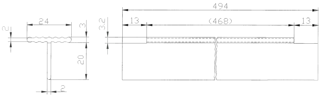
Vertical connection profile "Sto-Verbindungsleiste PVC" (dimensions in millimetres)
