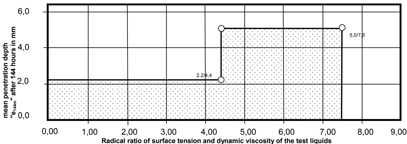
Figure 1: Penetration behavior (mean penetration depth "e 144m " of liquids) 1) on the basis of the respective dynamic viscosity and surface tension of the test liquids.
