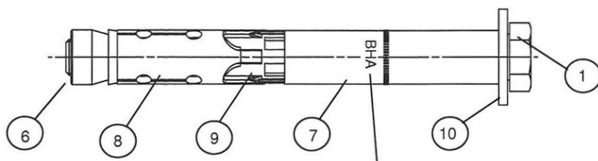
Screw type S BHA 10 - 32
