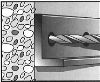
Drill hole with drill hammer
