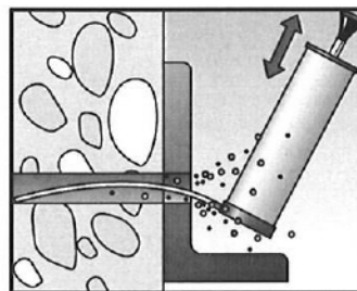
Blow out debris completely
