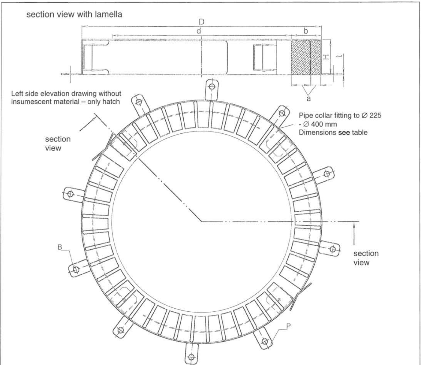
pipe collar "AWM II"
