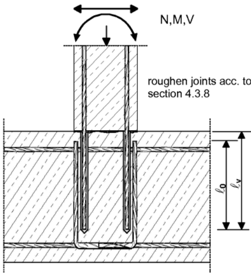
Figure 2: Overlap joint in a foundation of a column or wall where the rebars are stressed in tension
