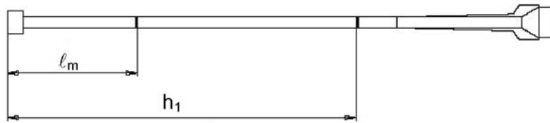
Figure 8: Marking lengths \ell_m on extension pipe for injection of adhesive
