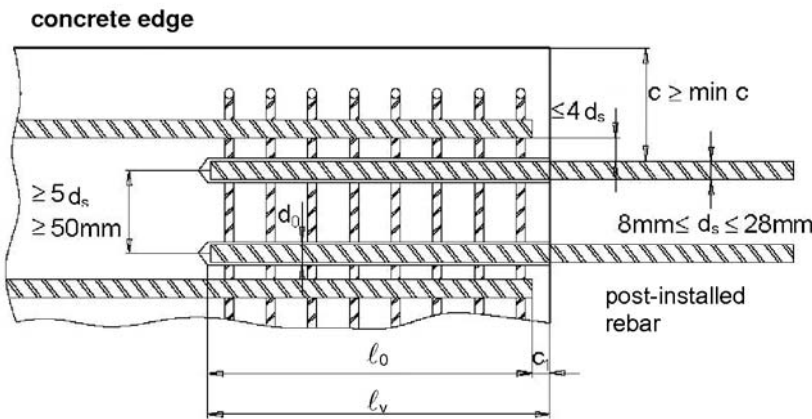
Figure 7: General rules for post-installed rebar connections
