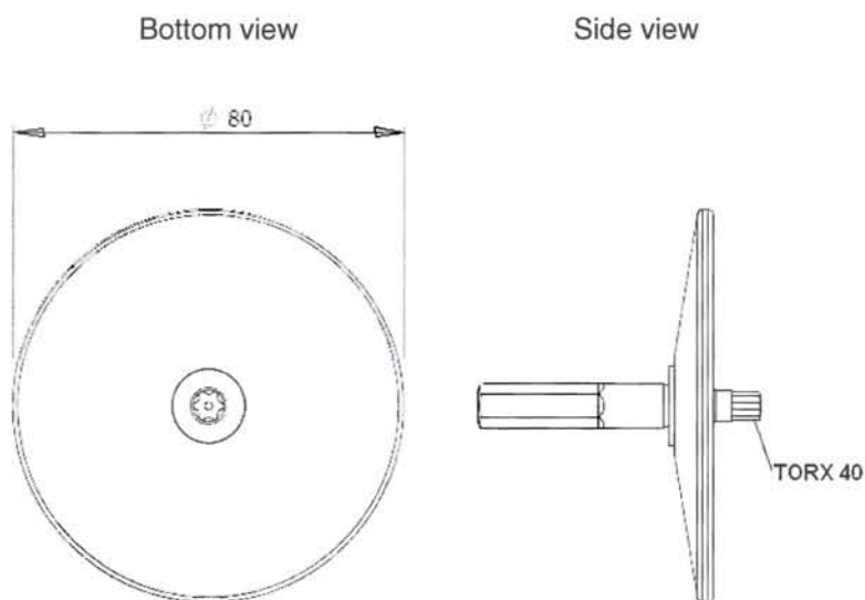
Drawing of setting device for TFIX-8ST
