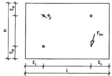
Figure 10: Moment from strain load F Zw in case of uniform bearing (Panel is fixed on 3 points)
