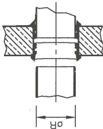
Detail X: Rohranschlüsse
