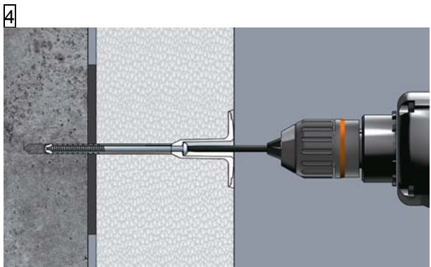
Surface fixed installation with STR-tool or standard bit
