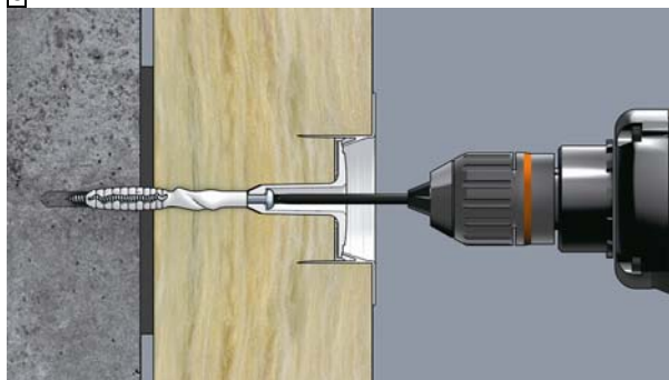
Mounting on the surface with STR-tool
