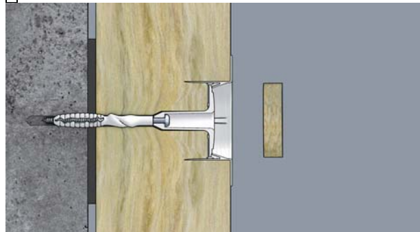
Insert the ejotherm STR cap
