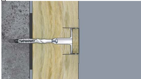
Installed anchor
