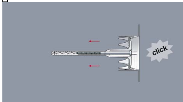
Assemble anchor and plate VT 2G
