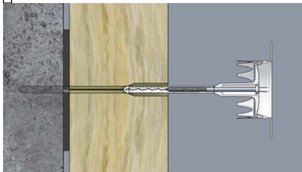
Insert the anchor into the drill hole
