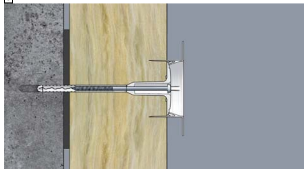
Drive through VT 2G until plate rests on surface
