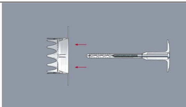
Assemble anchor and plate VT 2G
