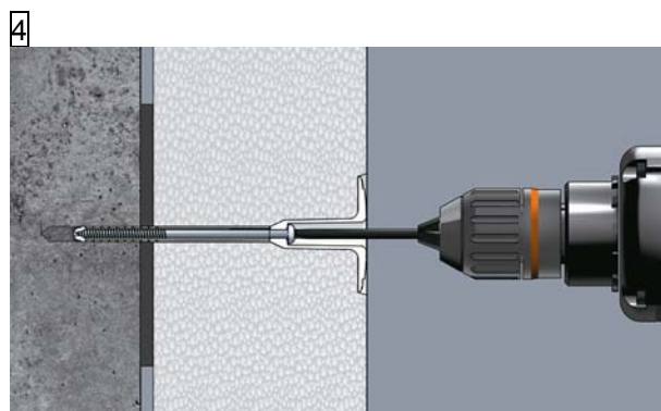
3 4 Surface fixed installation with STR-tool
