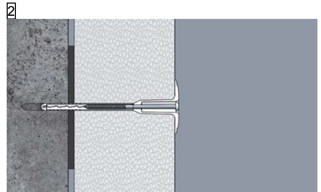
2 Insert the anchor
