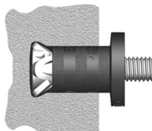
Stand-off fixing (carbon sleeve)
