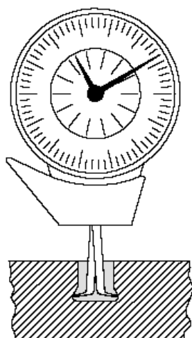
Dial gauge
