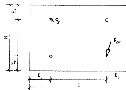
Figure 10: Moment from restraint F_{Zw} in case of uniform bearing (Panel is fixed on 3 points)
