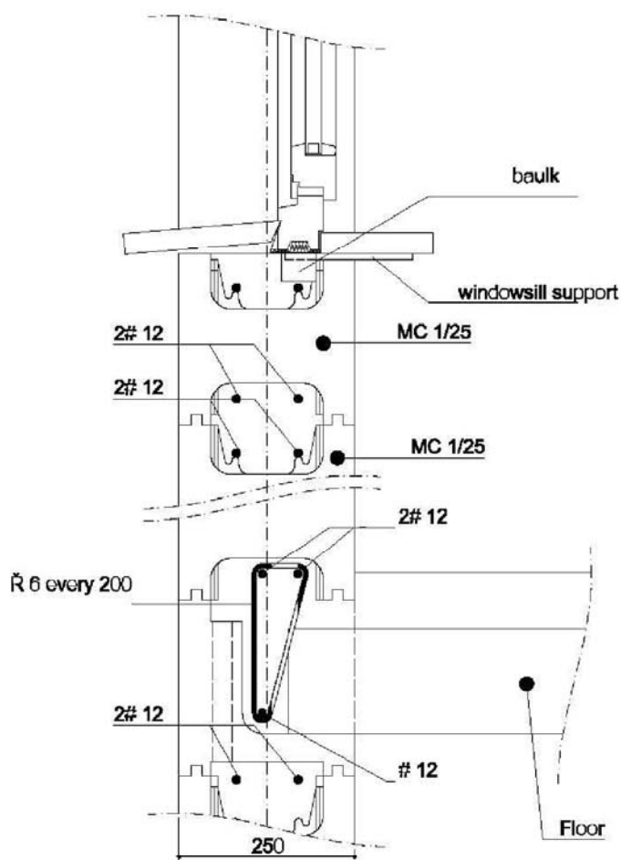
FASTENING OF SIDE WINDOW FRAME – DETAIL
