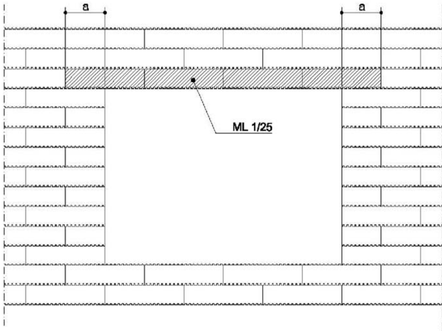
HEADER BLOCK LOCATION DIAGRAM ML 1/25
