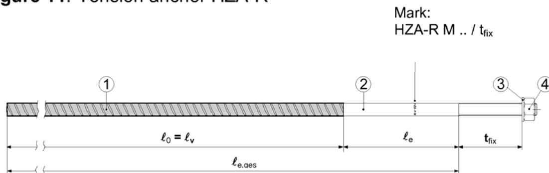
Figure 11: Tension anchor HZA-R
