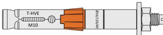
Anchor type HVE02 with threaded stud
