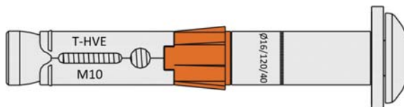
Anchor type HVE04 with mushroom head screw
