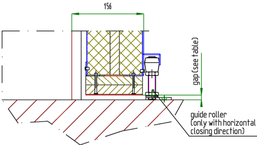
closing edge (installation closing at the bottom)
