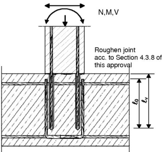
Figure 2: Overlap joint at a foundation of a column or wall where the rebars are stressed in tension
