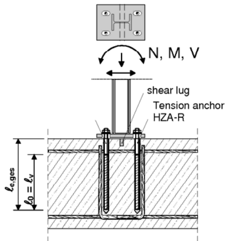
Figure 8: Overlap joint for the anchorage of cantilever members
