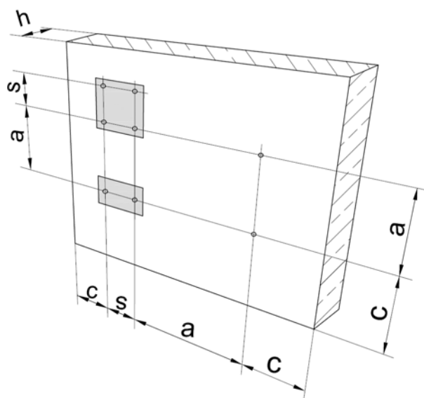
Scheme of distances and spacings in concrete
