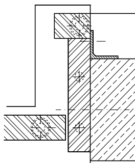
Joint at the top
