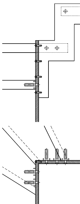
Joint at the top
