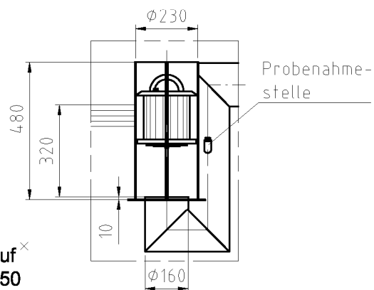
Detail Z
