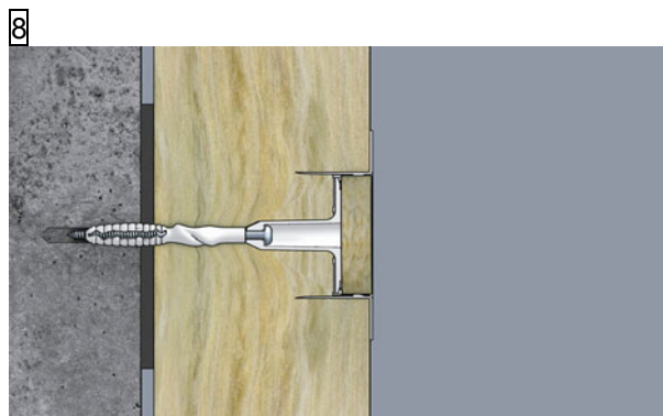
Installed anchor
