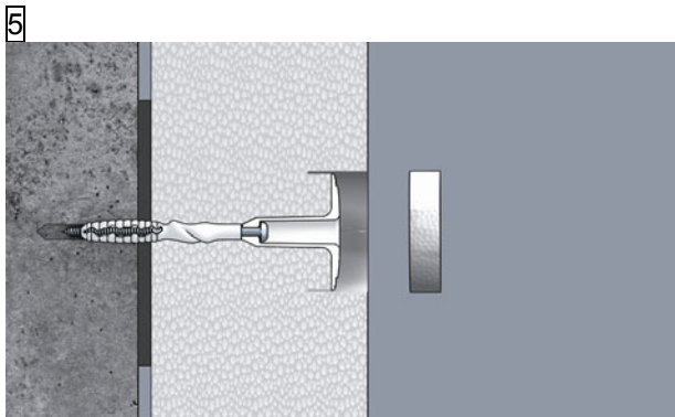
Insert the ejotherm STR cap with the help of a float
