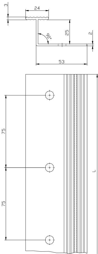
Horizontal profil – "Sto-Halteleiste PVC" (dimensions in millimetres)
