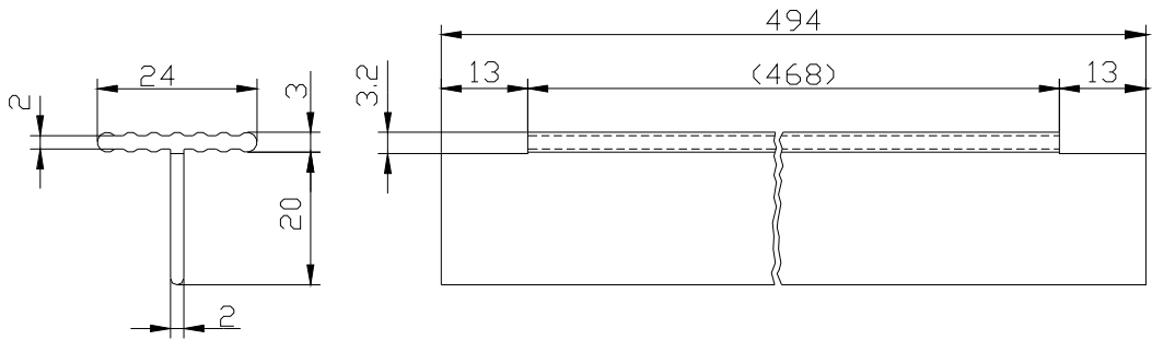
Vertical connection profil "Sto-Verbindungsleiste PVC" (dimensions in millimetres)
