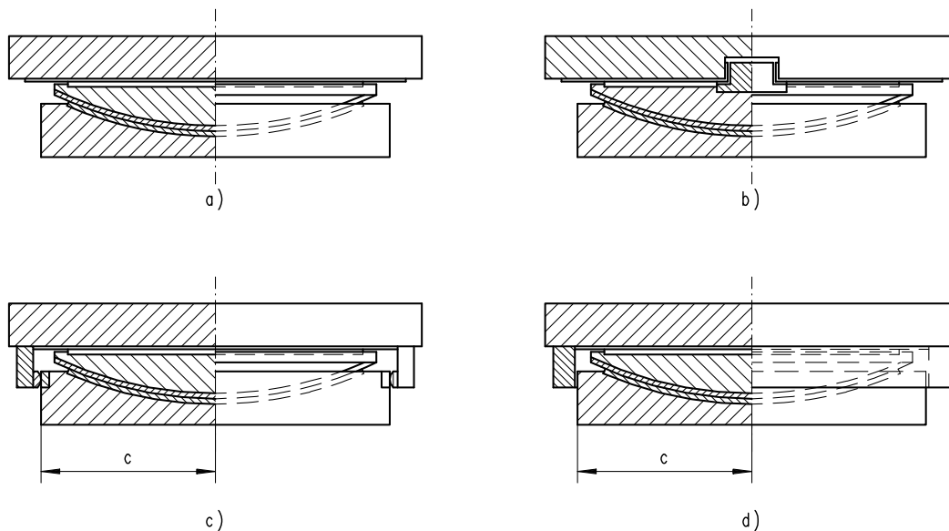
Figure A.2 - MAURER MSM ® spherical bearings
