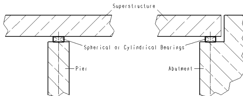
Figure A.1 - Assembly of a guided and free movable spherical or cylindrical bearing with MSM® and its intended use
