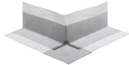
Type "NVV" leg length 75 or 140 mm
