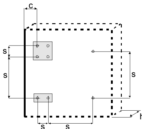
Scheme of distance and spacing in concrete
