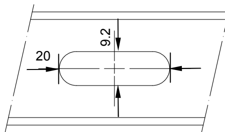
2. slotted hole: at panel load-bearing profile (skid)
