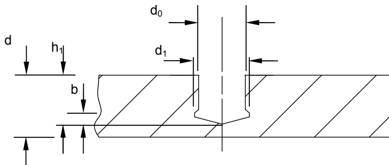
2. drill hole geometry
