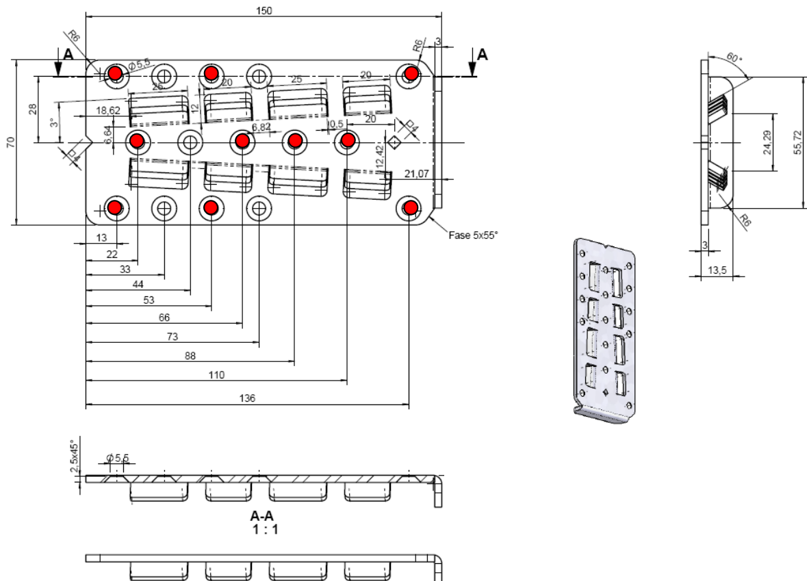
Figure A.6 Header plate of the beam connector 150 x 70 (● screws for column connection)
