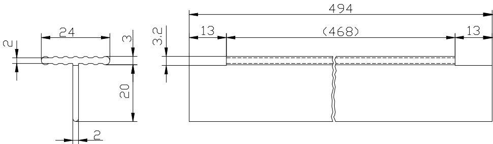
Vertical connection profile "HAERING Verbindungsleiste PVC" (dimensions in millimetres)
