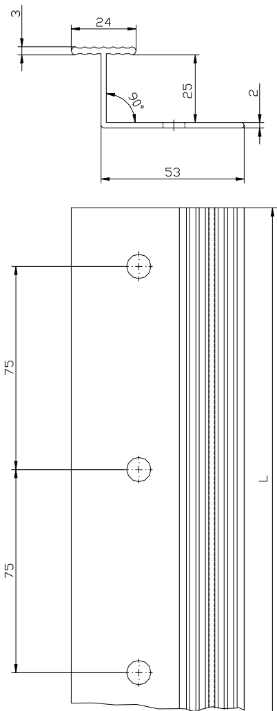
Horizontal profile – "HAERING Halteleiste PVC" (dimensions in millimetres)
