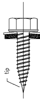
self tapping screw with sealing washer
