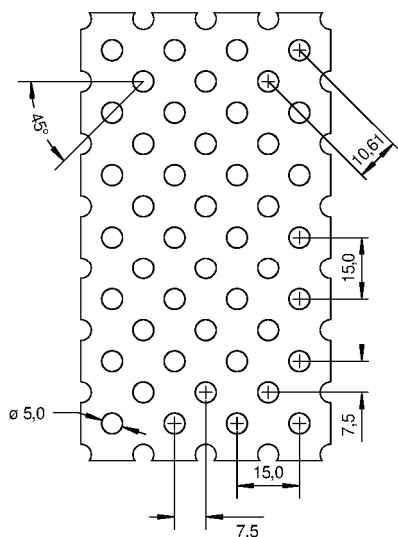
Hole pattern II
