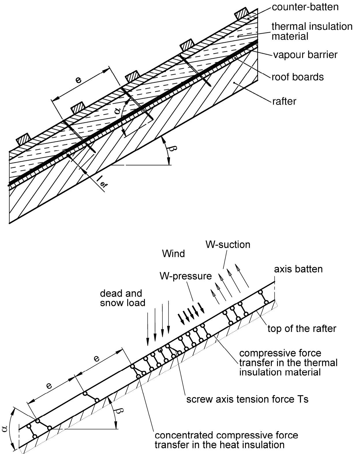
Figure 3.1 Fastening of the thermal insulation material on top of rafters - structural system for parallel inclined screws
