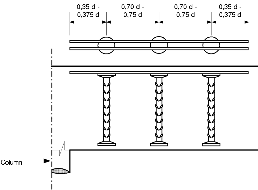
Three-anchor element
