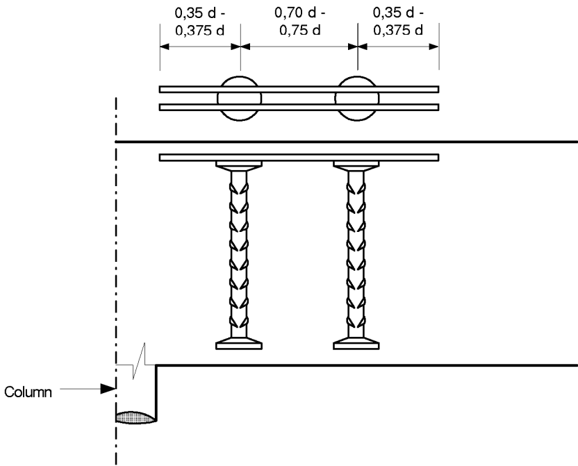
Two-anchor element
