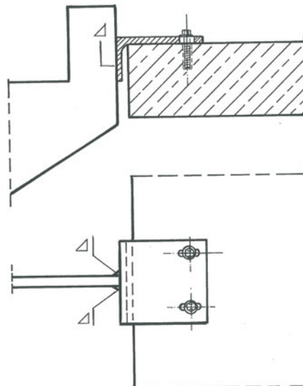
Joint at the top
