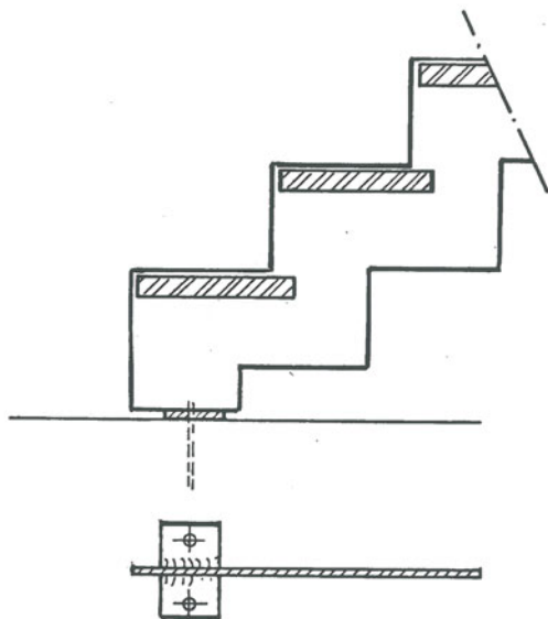
Joint at bottom
